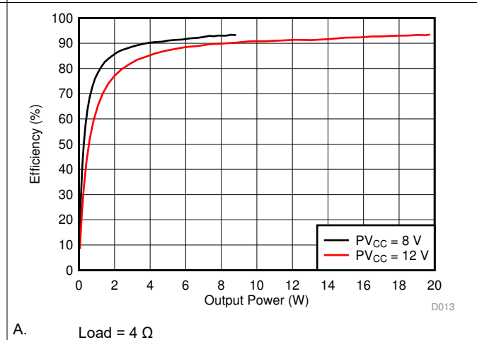
Figure 6-27. Efficiency vs Output Power, 4 \Omega
