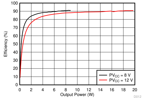
Figure 6-8. Efficiency vs Output Power (BTL)
