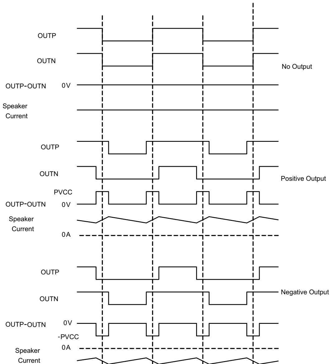
Figure 7-2. BD Mode Modulation
