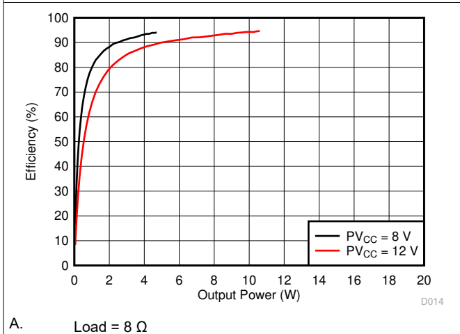
Figure 6-26. Efficiency vs Output Power, 8 \Omega
