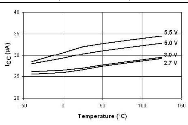
Figure 43. I_{CC} vs. temperature (enabled) (STMPS2161/2171)
