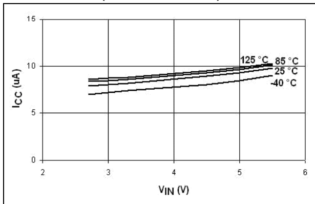
Figure 44. I_{CC} vs. V_{IN} (disabled) (STMPS2161/2171)
