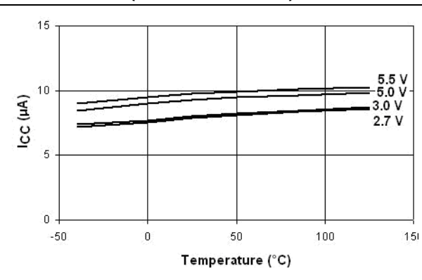
Figure 45. I_{CC} vs. temperature (disabled) (STMPS2161/2171)
