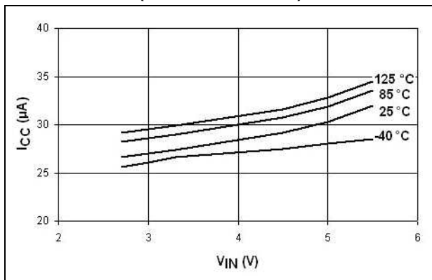
Figure 42. I_{CC} vs. V_{IN} (enabled) (STMPS2161/2171)
