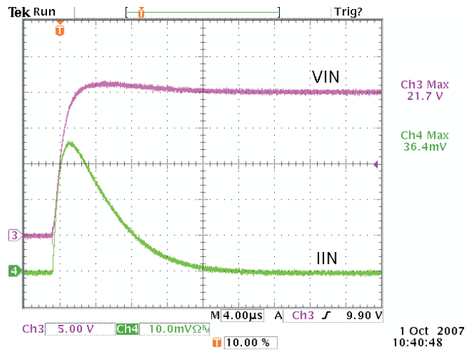
Figure 40. Adapter DC Side Hot Plug-in Test Waveforms
