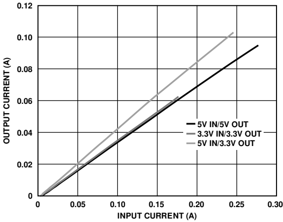
Figure 5. Typical Isolated Output Supply Current vs. External Load in All Supported Power Configurations
