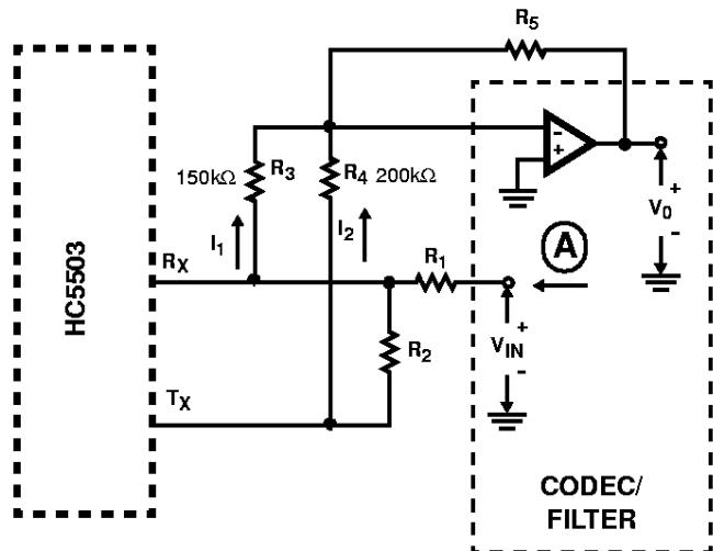
FIGURE 6. TRANSHYBRID CIRCUIT
