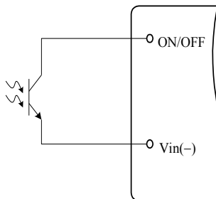
Figure 9. Opto Coupler Enable Circuit
