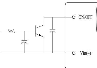
Figure 10. Open Collector Enable Circuit
