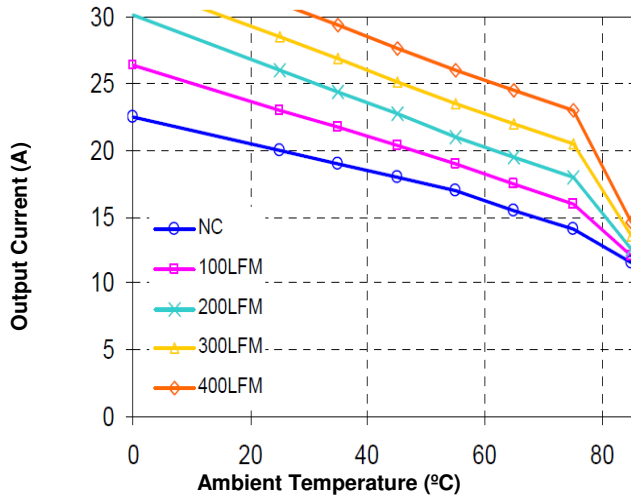
Figure 7. Current Derating Curve with Open Frame (Direction 3 (Ref. Figure 8); typical Vin, socket interface)
