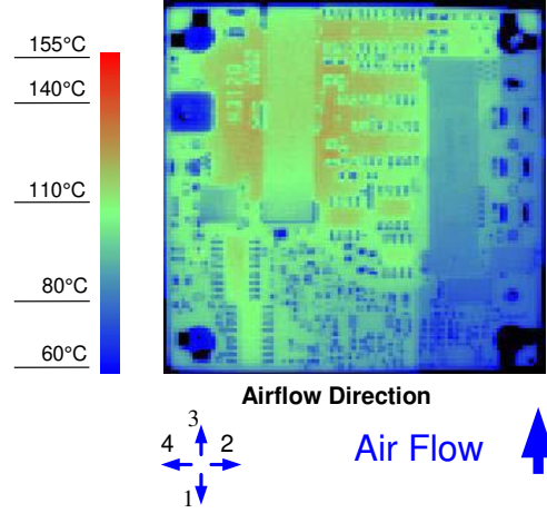
Figure 8. Thermal Image for Airflow Direction 3 (26A output, 55°C ambient, 200 LFM, typical Vin, open frame, socket interface)
