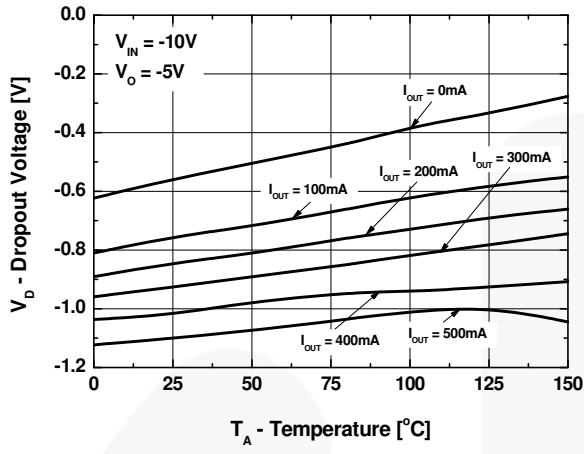
Figure 2. Dropout Voltage
