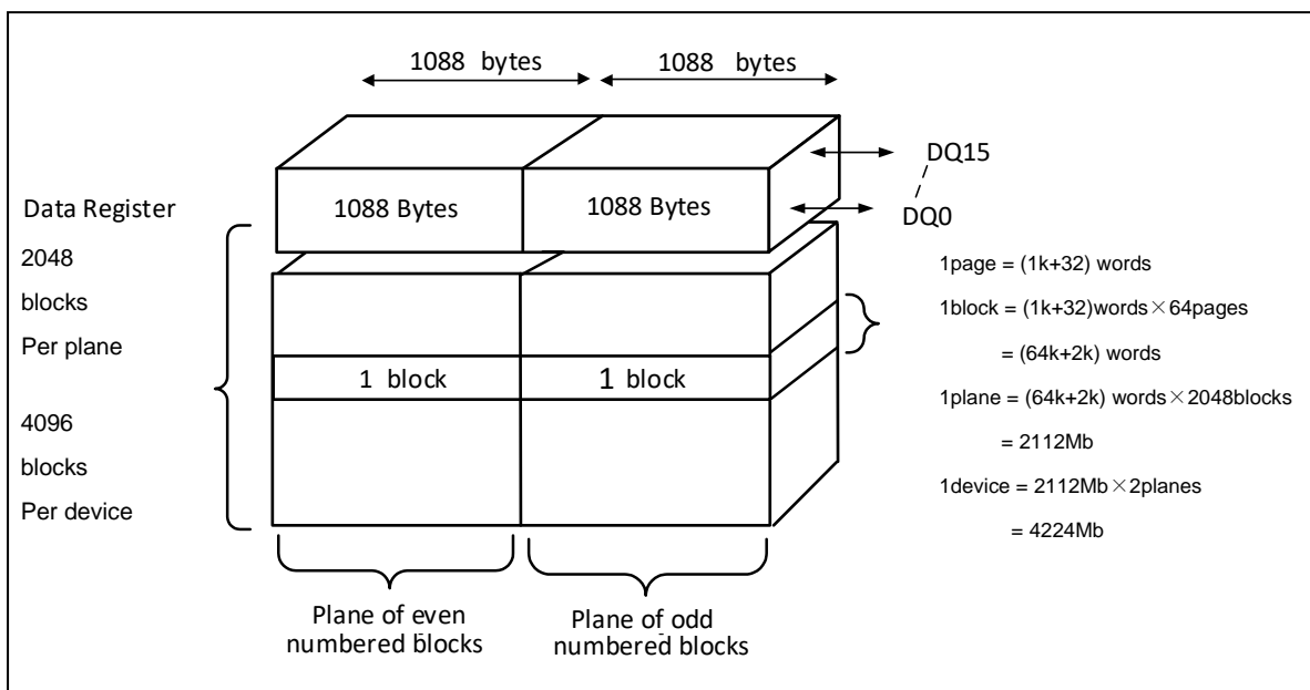
Figure 6-2 Array Organization (x16)
