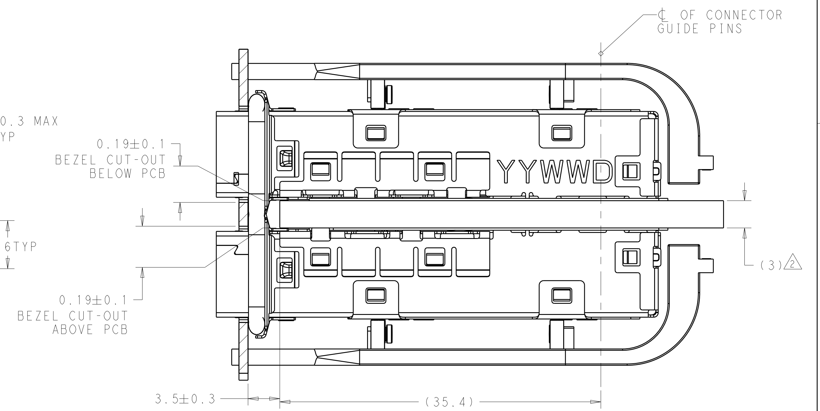
MOUNTED BELLY TO BELLY ON PC BOARD SHOWN THRU RECOMMENDED BEZEL SCALE 4:1
