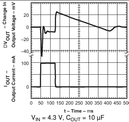
Figure 26. TPS79118 Load Transient Response
