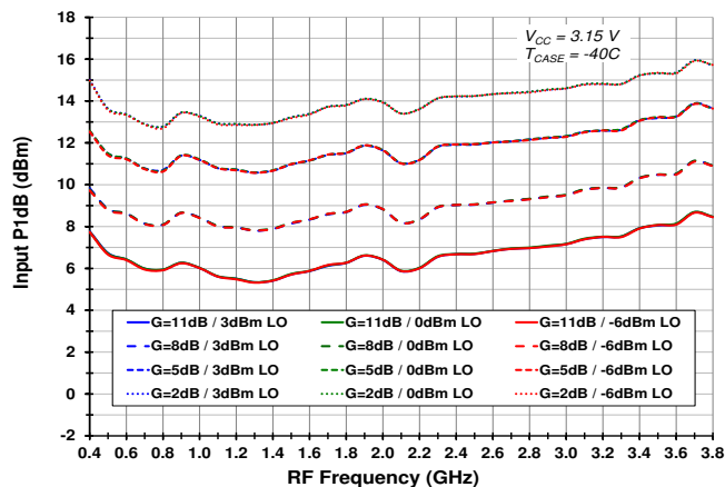
Figure 10. Input P1dB vs. LO Level and Gain Setting ( V_{CC} = 3.15 , T_{CASE} = -40^{\circ}C )
