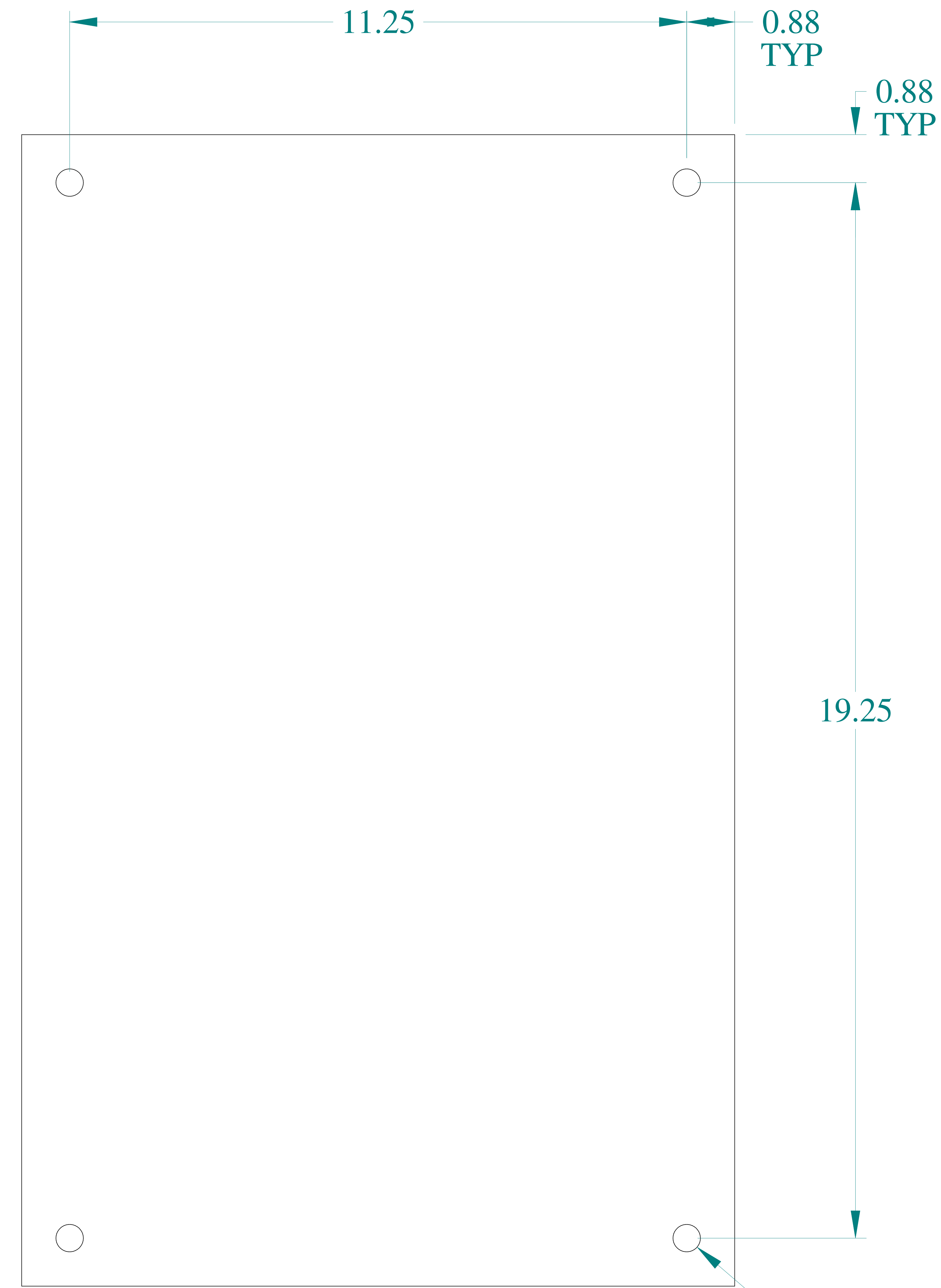
FRONT VIEW
