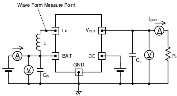
< Circuit No.① >
