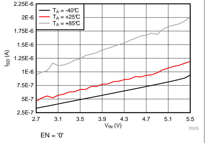
Figure 6. Shutdown Current
