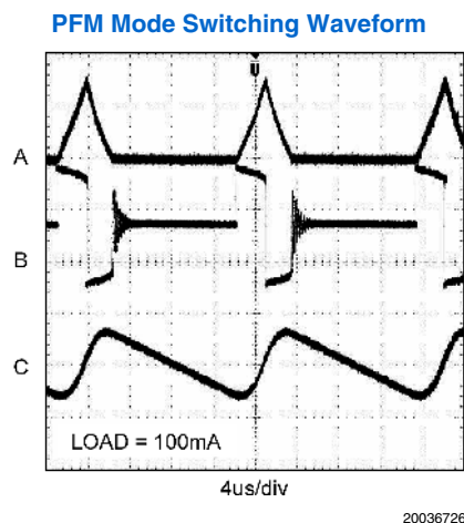
A: Inductor Current, 500mA/div B: SW Pin, 2V/div C: V_{OUT} , 50mV/div, AC Coupled
