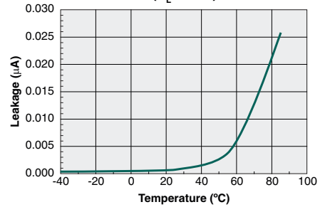
Typical Leakage vs. Temperature Measured Across Pins 3&4 ( V_L=400V )
