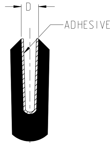
PART AS SUPPLIED
