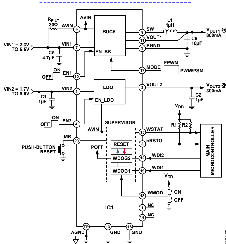
Figure 56. Application Diagram
