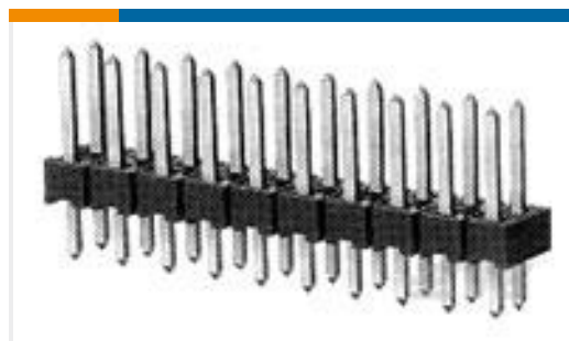
TE Part #5-146257-7 14 MODII HDR DRST B/A .100CL L
