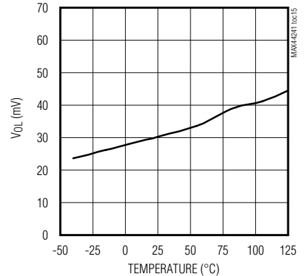
OUTPUT VOLTAGE LOW vs. TEMPERATURE
