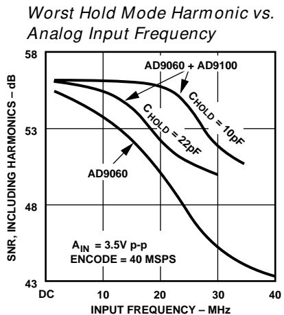
SNR vs. Analog Input
