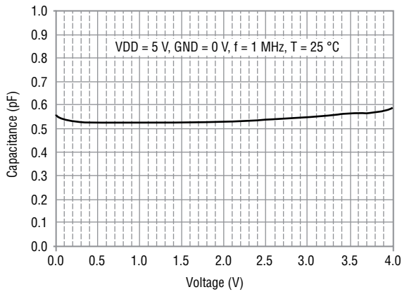
Typical Variation of C_{IO \text{ to } IO} vs. V_{IN}
