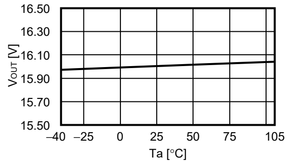
6.4 V_{OUT} = 16.0\text{ V}
