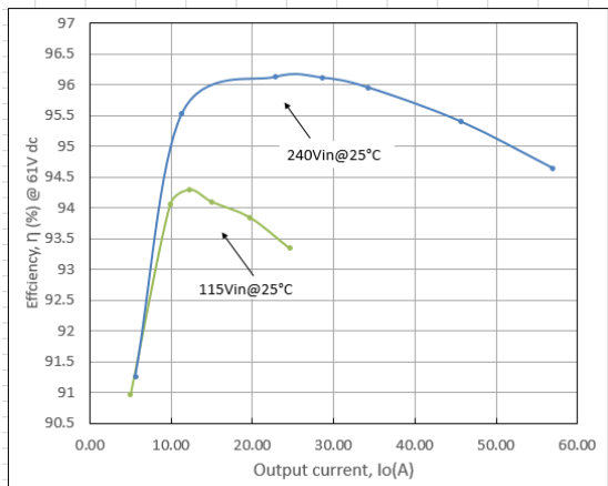
Figure 1. Power Supply Efficiency versus Output Current.
