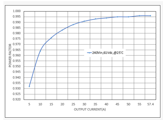
Figure 2. Power Factor versus Output Current
