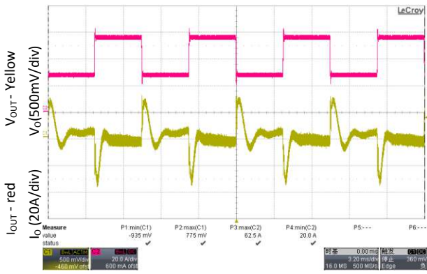
Figure 7. Transient response 65V DC load step 10 – 60%, Slew rate: 1A/μs, V IN = 230V AC
