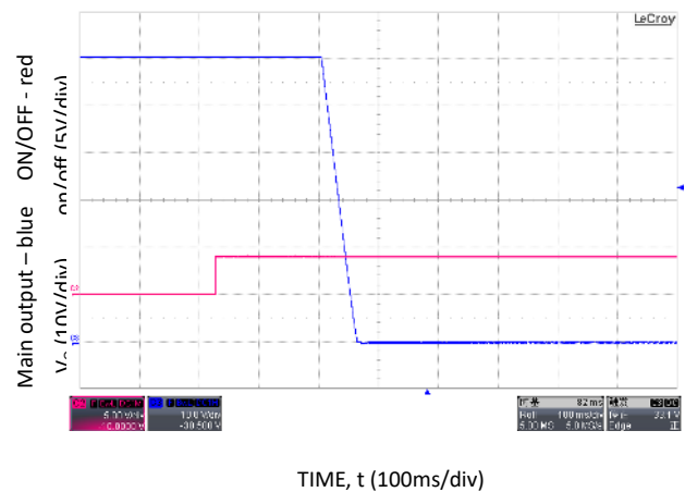
Figure 16. 65V DC turn-OFF delay when ON/OFF is di-asserted, V_{IN}=230V_{AC} - I 2 C mode.
