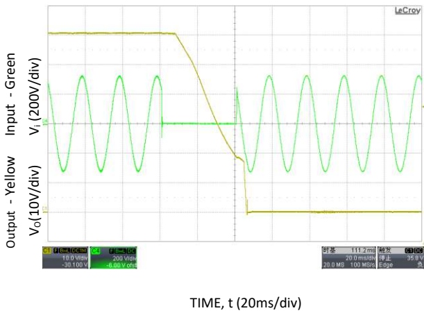
Figure 13. 40ms AC dropout @ full load, V_{IN} = 230V_{AC} .
