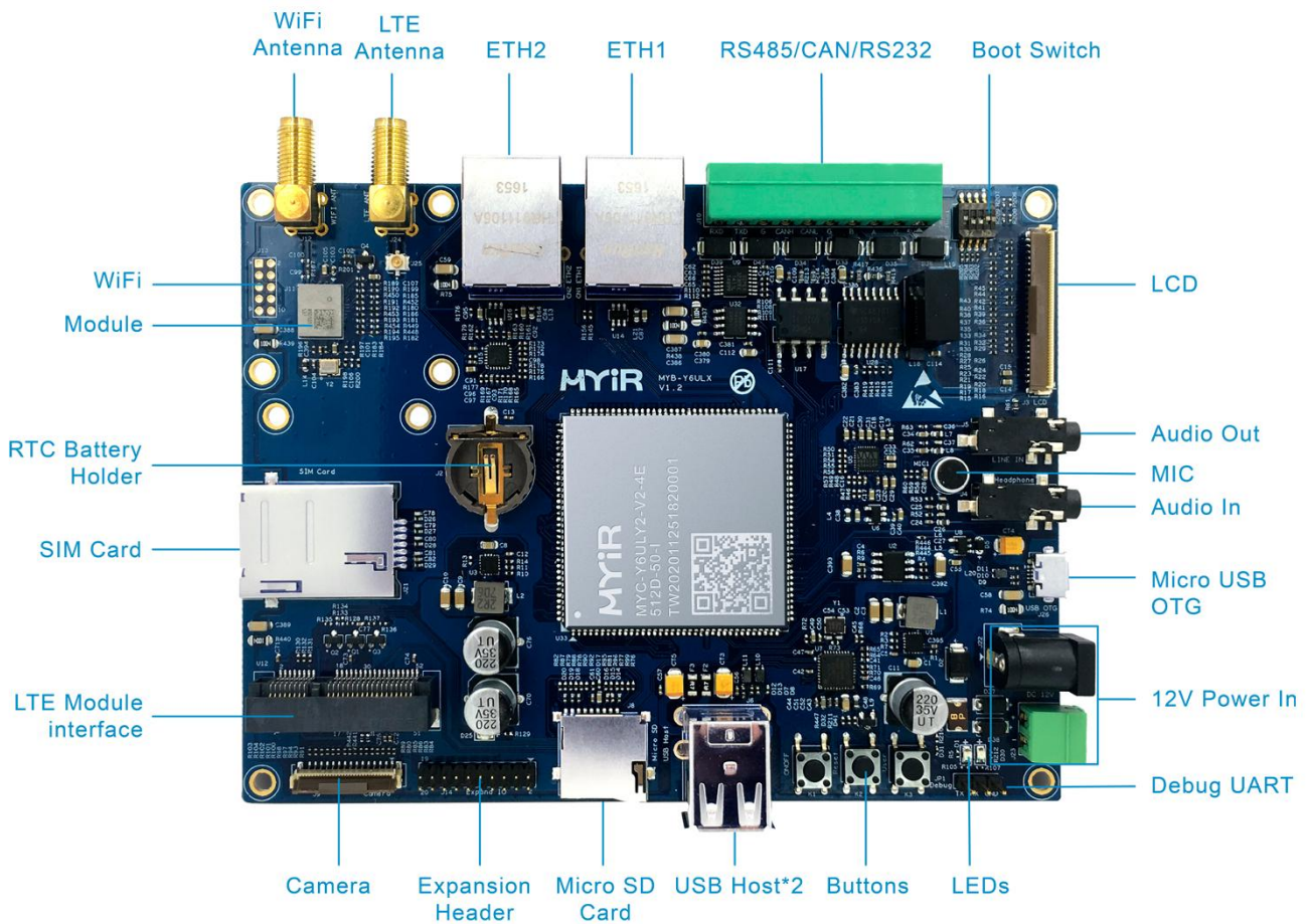
Figure 1-2 MYD-Y6ULX-V2 Development Board Interface Diagram
