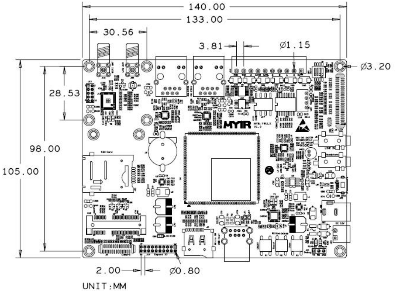
Dimension Chart of MYD-Y6ULX-V2
