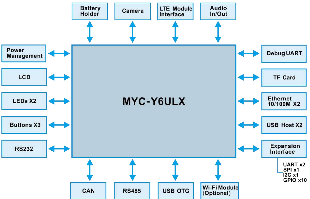
MYD-Y6ULX-V2 Function Block Diagram
