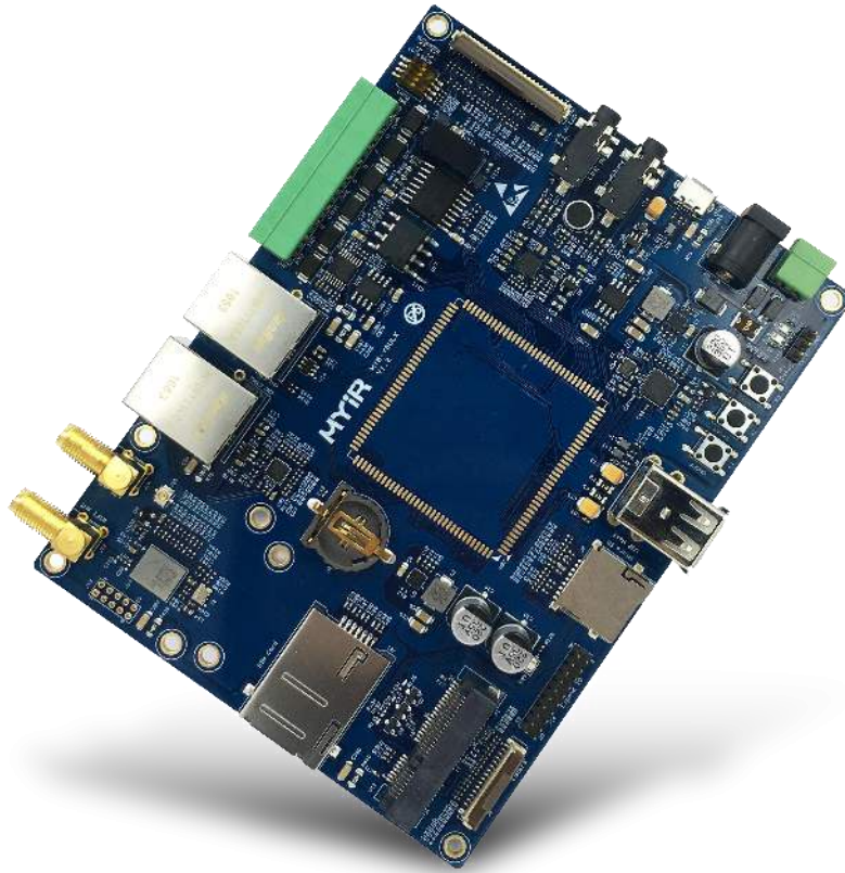
MYD-Y6ULX-V2 Base Board
