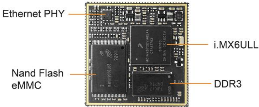
MYC-Y6ULX-V2 CPU Module (delivered with shielding cover by default)
