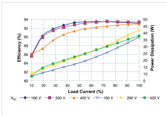
Figure 11 — V_{IN} to V_{OUT} efficiency and power dissipation vs. V_{IN} to I_{OUT} , T_{CASE} = 25^\circ\text{C}
