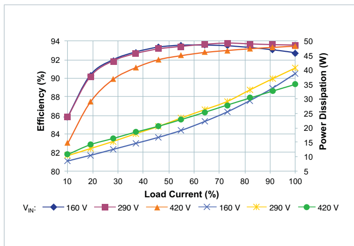
Figure 10 — V_{IN} to V_{OUT} efficiency and power dissipation vs. V_{IN} to I_{OUT} , T_{CASE} = -40^\circ\text{C}
