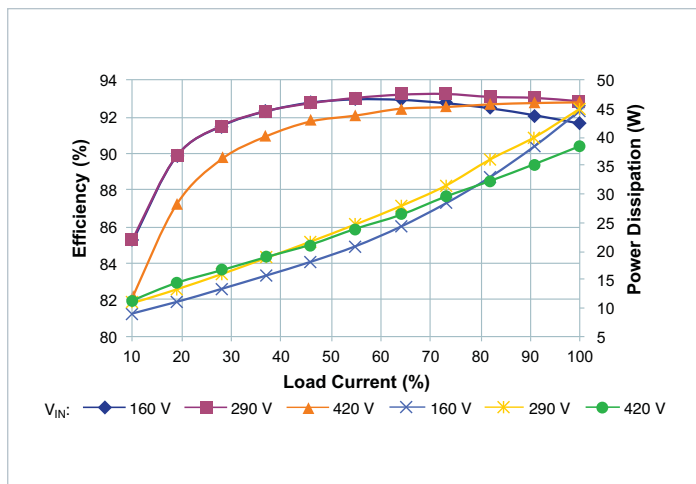
Figure 12 — V_{IN} to V_{OUT} efficiency and power dissipation vs. V_{IN} to I_{OUT} , T_{CASE} = 90^\circ\text{C}
