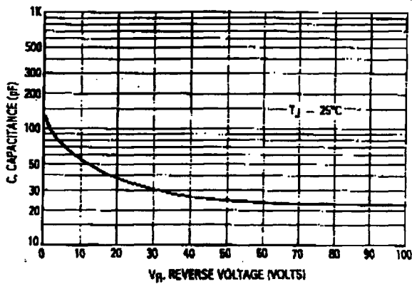
Figure 8. Typical Capacitance
