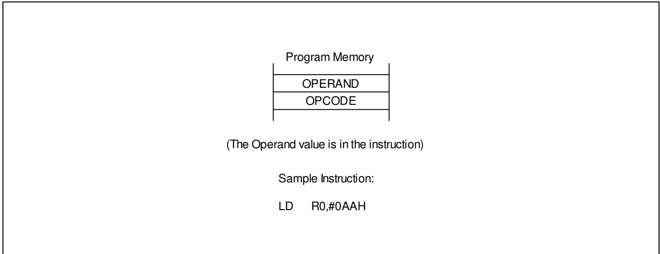
Figure 3-14 Immediate Addressing
