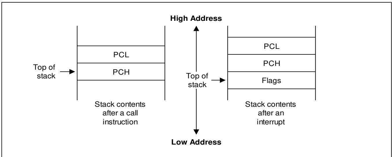
Figure 2-16 Stack Operations
