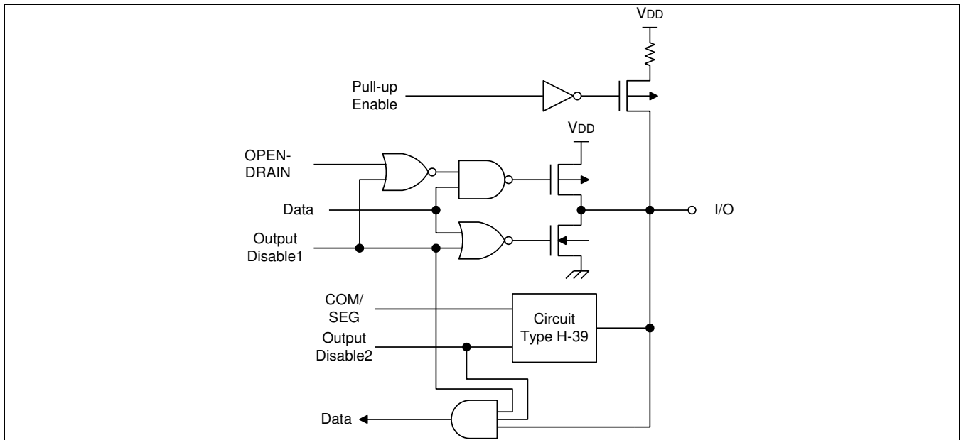
Figure 1-11 Pin Circuit Type H-42 (P4)
