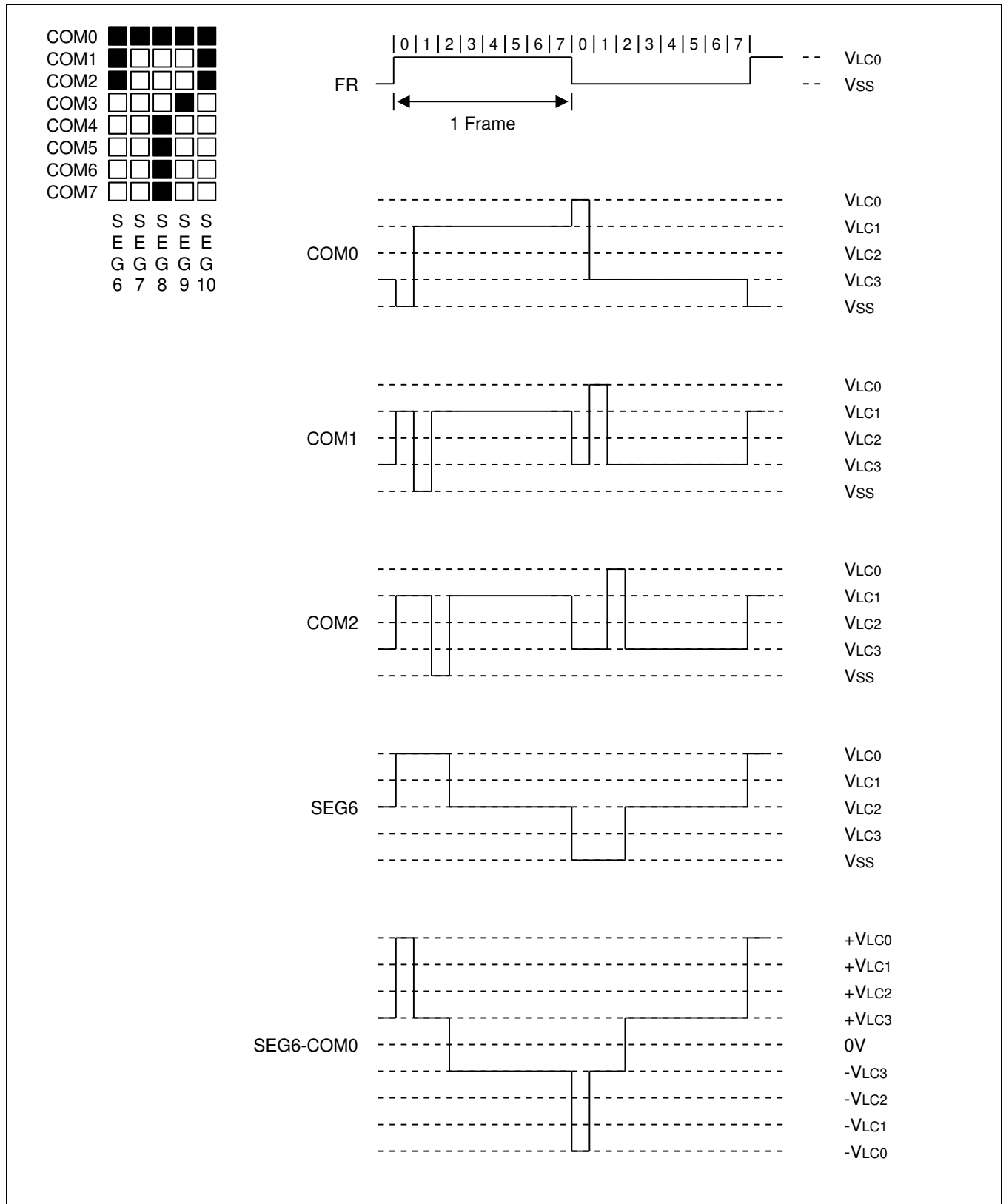
Figure 15-14 illustrates the LCD signal waveforms (1/8 Duty, 1/4 Bias).
