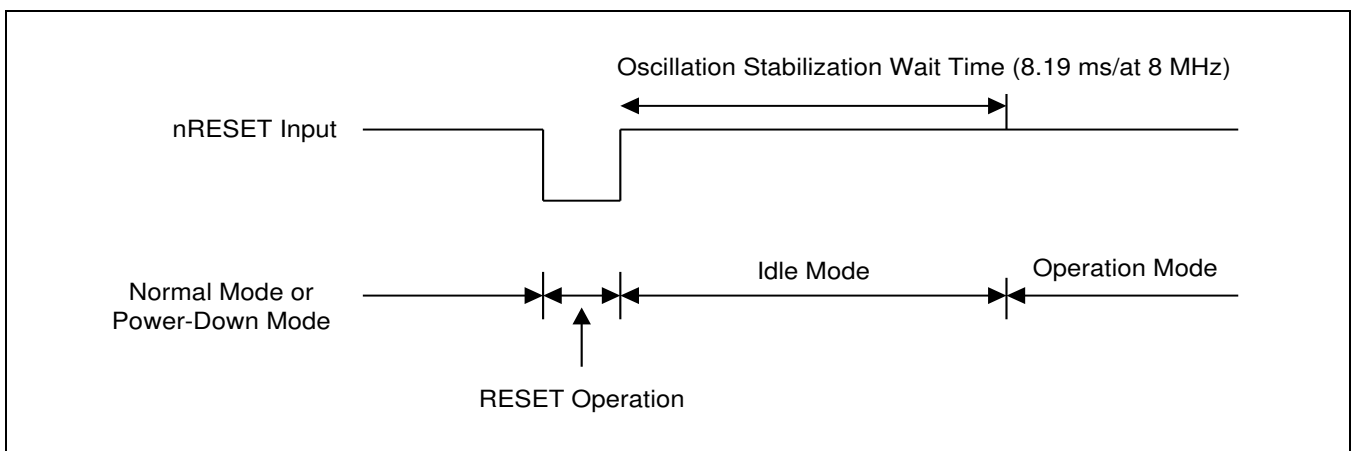
Figure 8-3 Timing for S3F8S19/S3F8S15 After RESET
