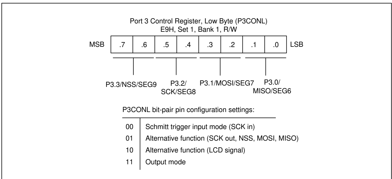
Figure 9-9 Port 3 Low-Byte Control Register (P3CONL)
