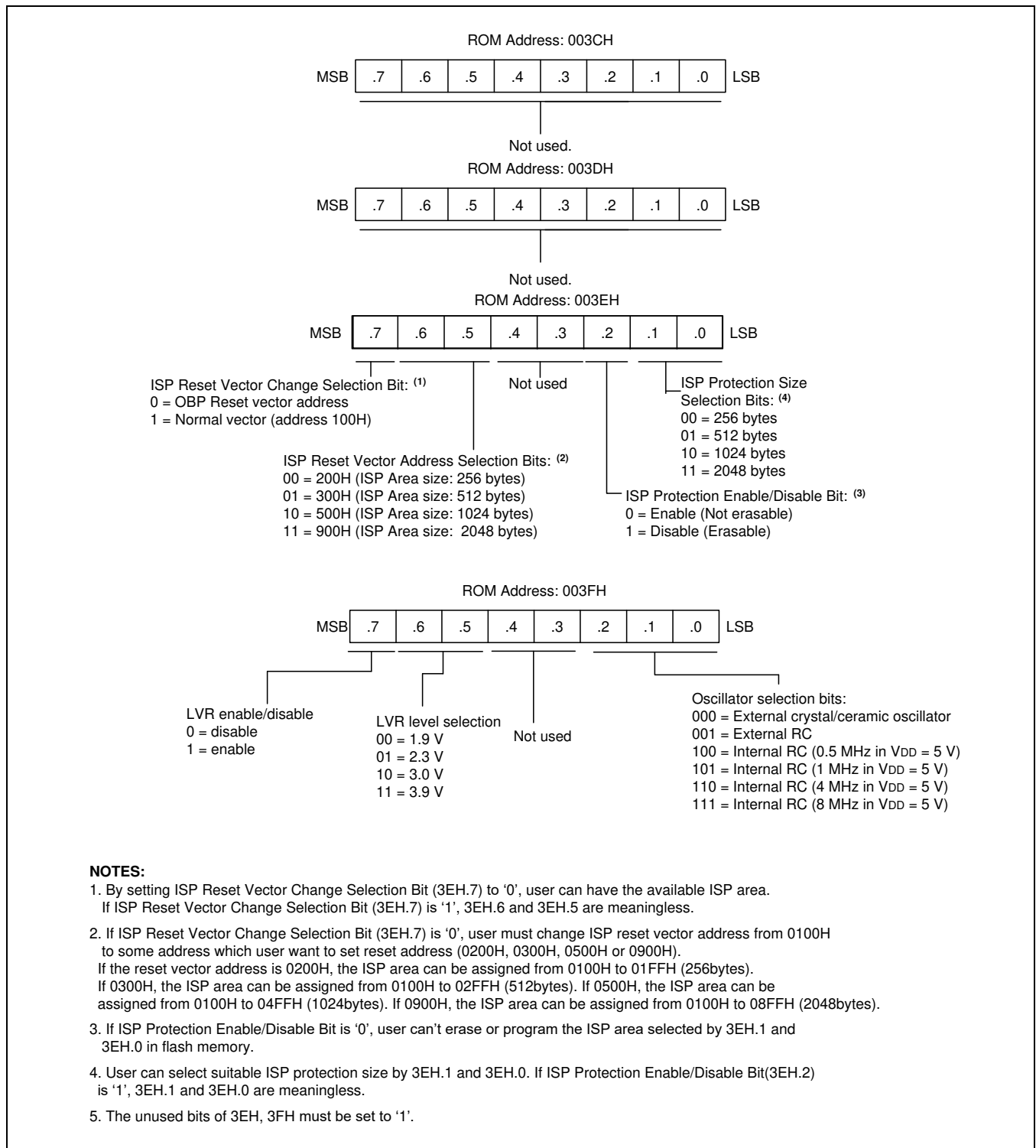
Figure 2-2 Smart Option
