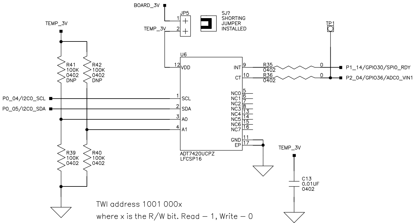
Figure 25. PC Temperature Sensor Circuit Diagram
