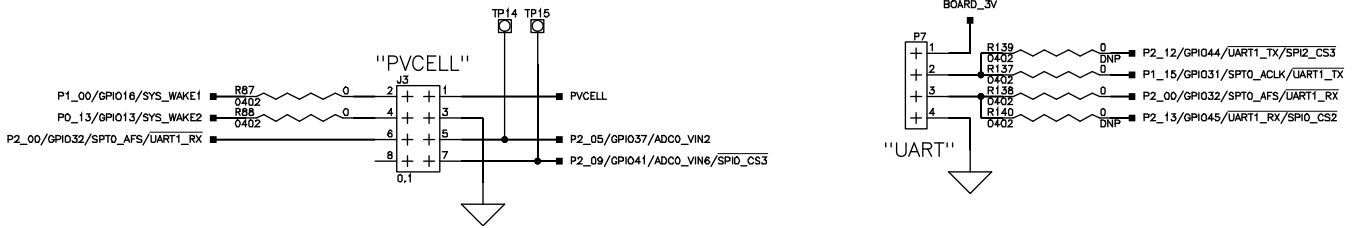
Figure 32. PV Cell Connector and UART (P7) Connector Schematic
