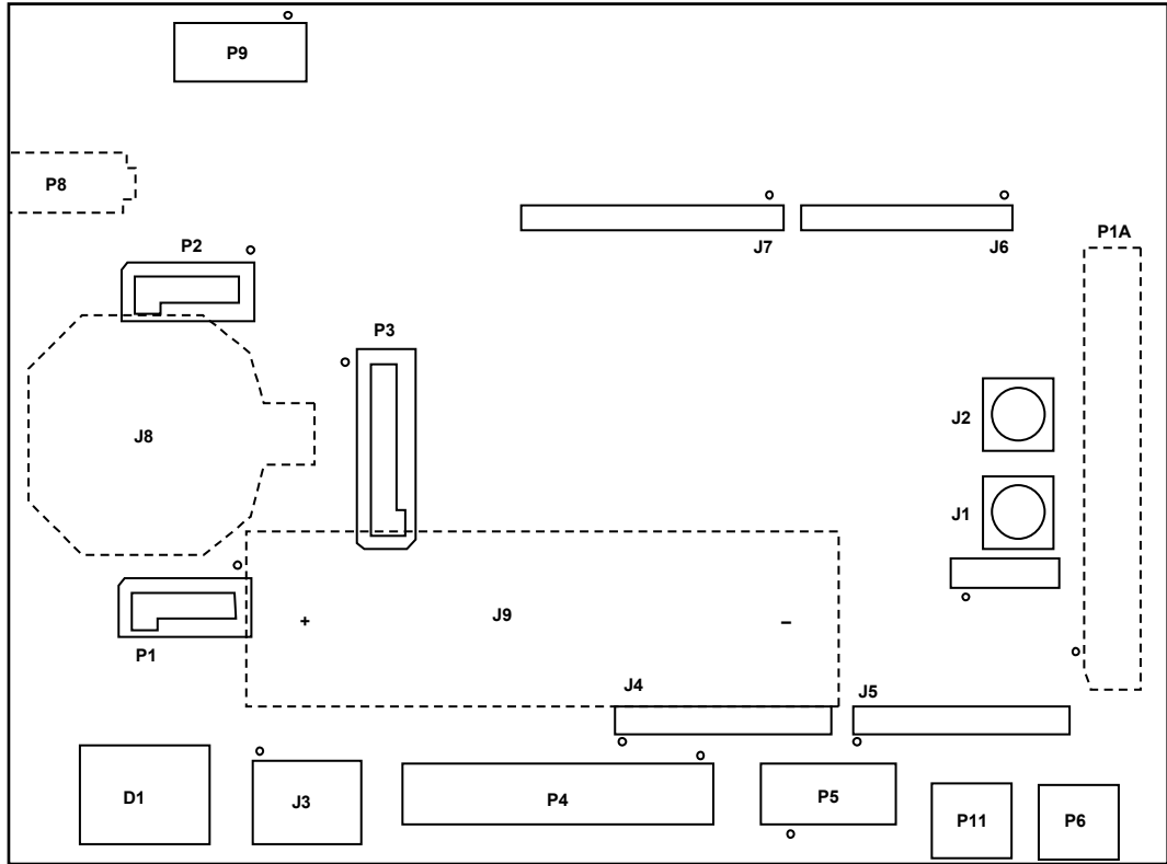
Figure 10. Connector Locations
