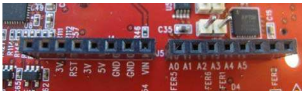
Figure 11. J4 and J5 Arduino Compatible Interface (Power and ADC)
