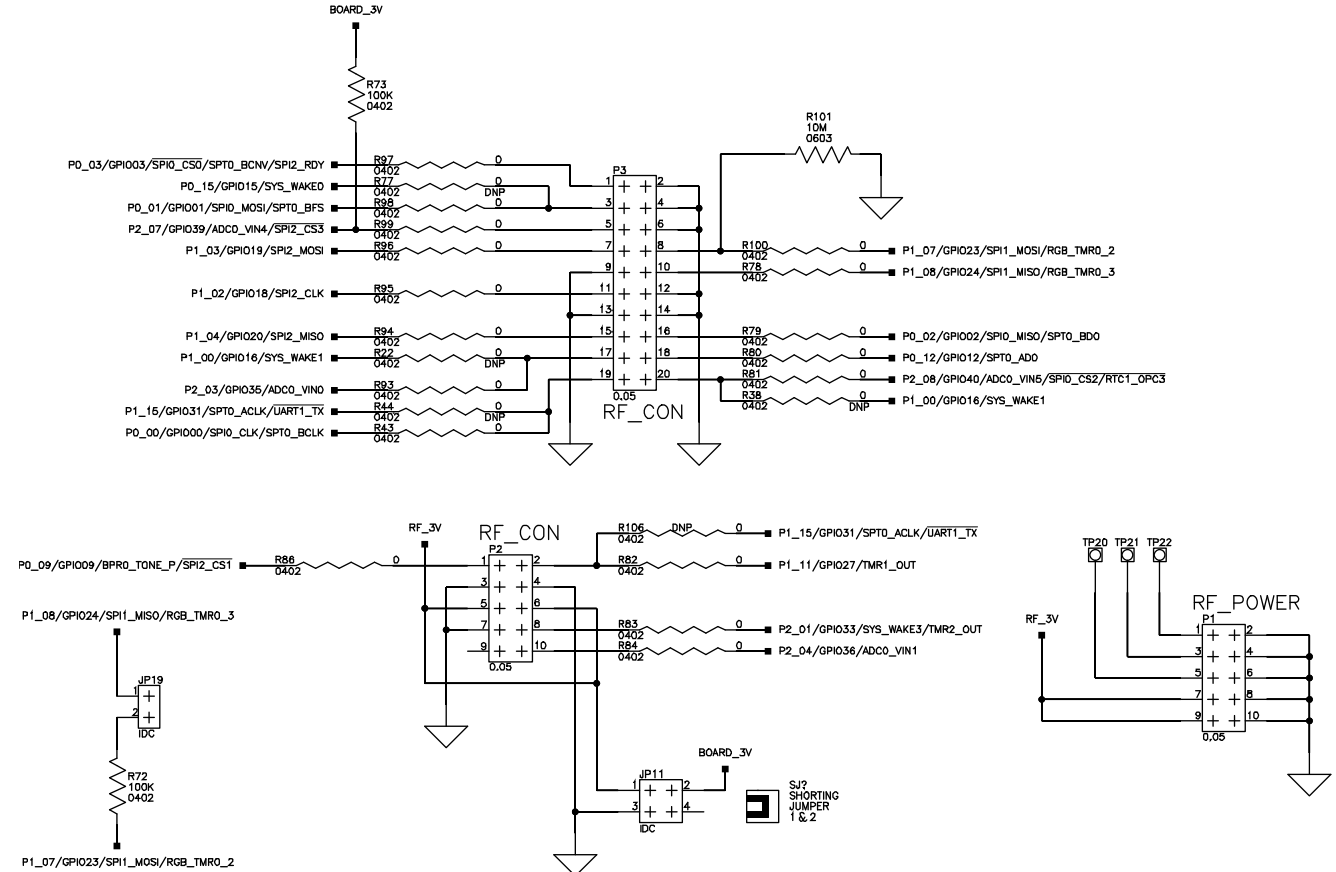
Figure 33. Wireless Transceiver Interface Schematic
