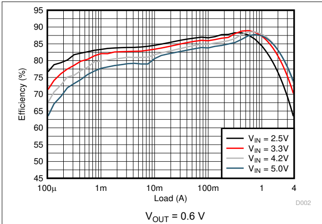
Figure 9-3. Efficiency
