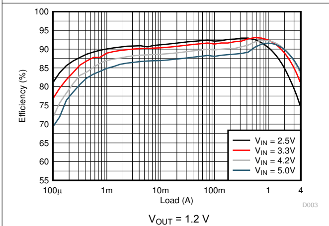
Figure 9-7. Efficiency
