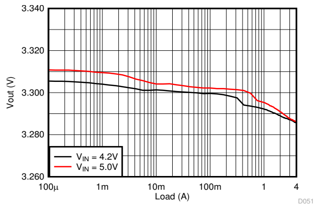
Figure 9-20. Load Regulation
