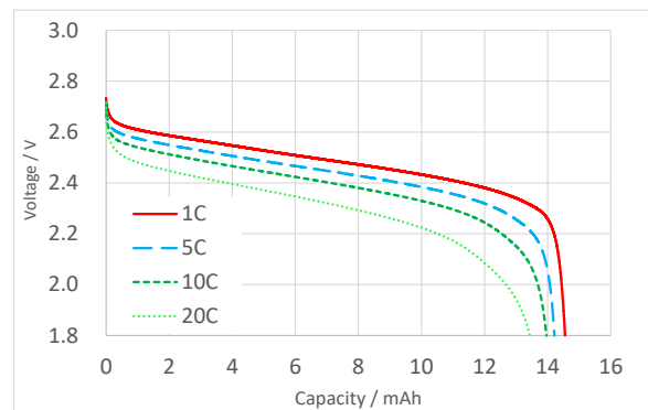
Discharge characteristics
