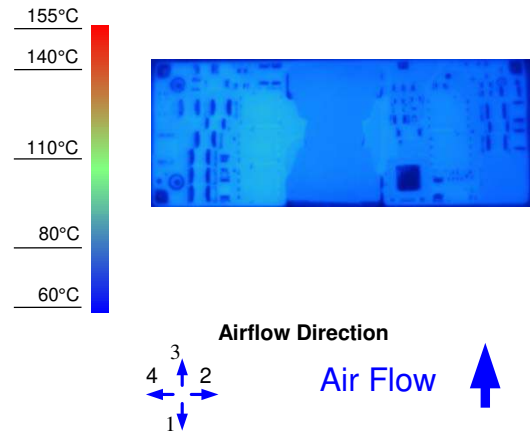
Figure 8. Thermal Image for Airflow Direction 3 (10A output, 55°C ambient, 200 LFM, typical V_{in} , open frame, socket interface)
