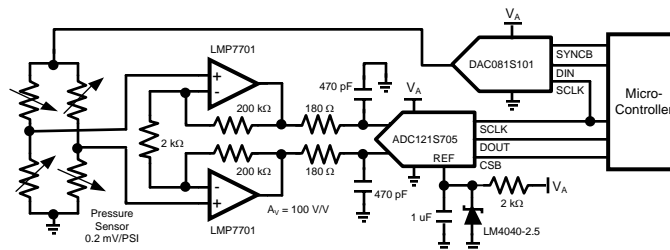
Figure 62. Interfacing the ADC121S705 for a Pressure Sensor
