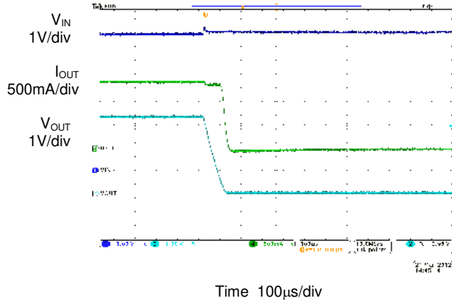
OVP Function ( V_{IN}=5V to 6V )
