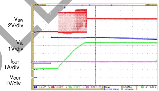
Time 200µs/div
