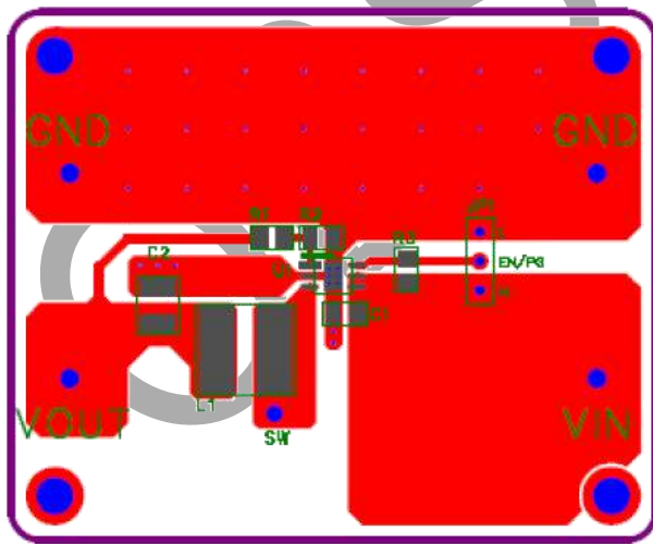
Figure 32. Top Layer for Demo Board
