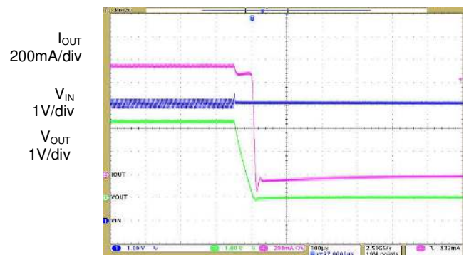
Time 100µs/div
