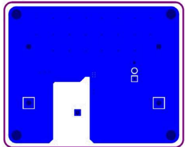
Figure 33. Bottom Layer for Demo Board
