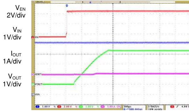
Time 200µs/div
