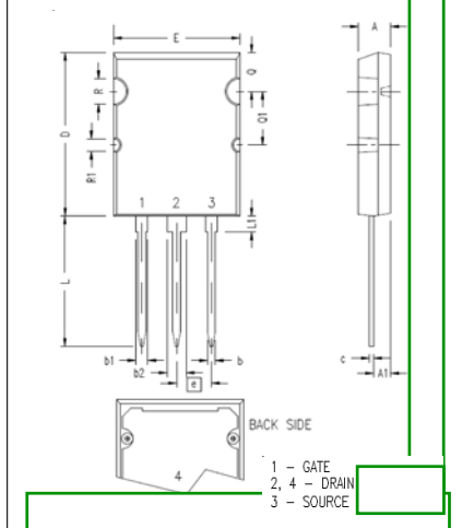
PLUS264™ (IXFB) Outline
