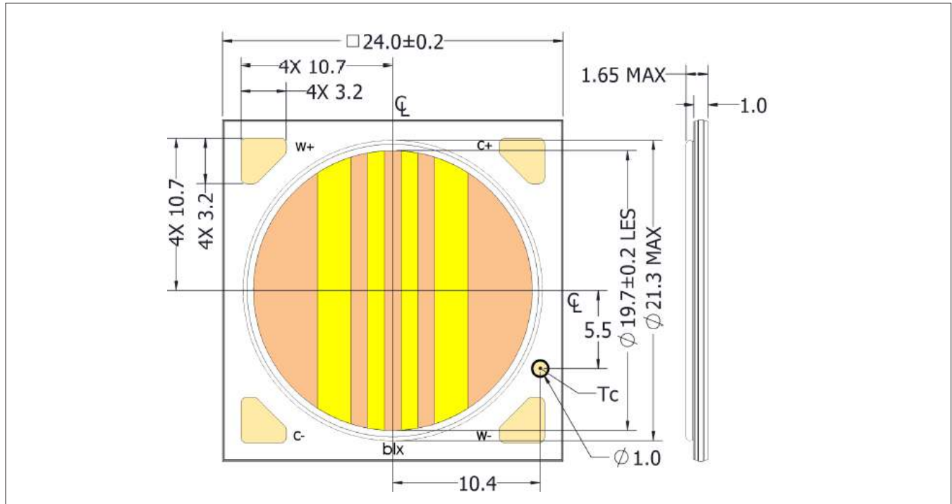
Figure 14: Drawing for Vesta Series Tunable White Gen 2 18mm Array
