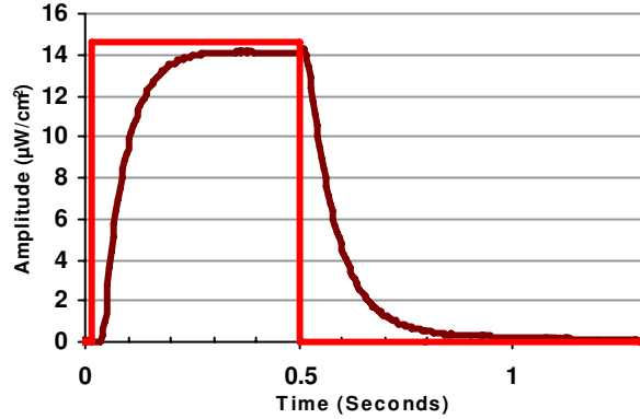
Load = 10kΩ and 1μF Photo Step = Direct Light Input of 14.6μW/cm²
