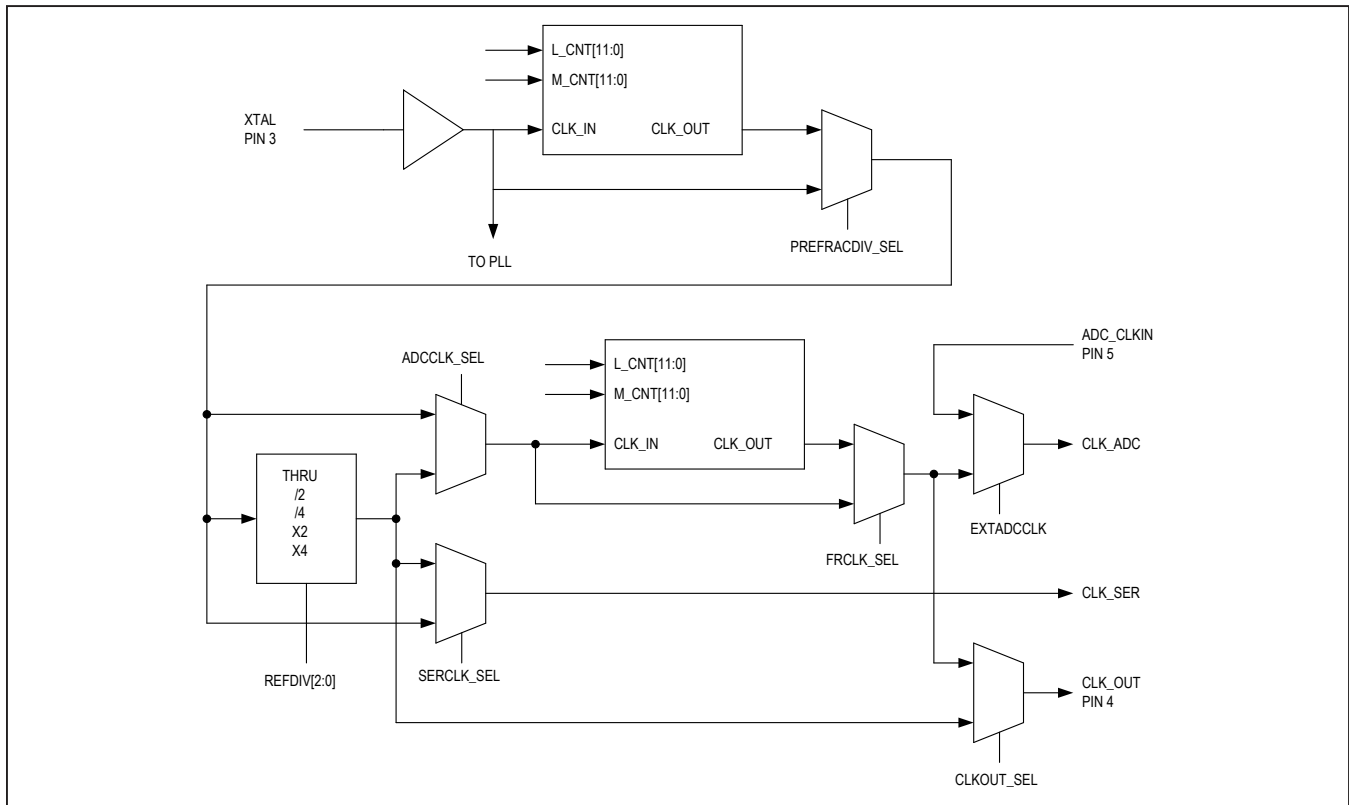
Figure 3. Clock Distribution
