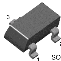
SOT-23 Mark: D2 1. Base 2. Emitter 3. Collector
