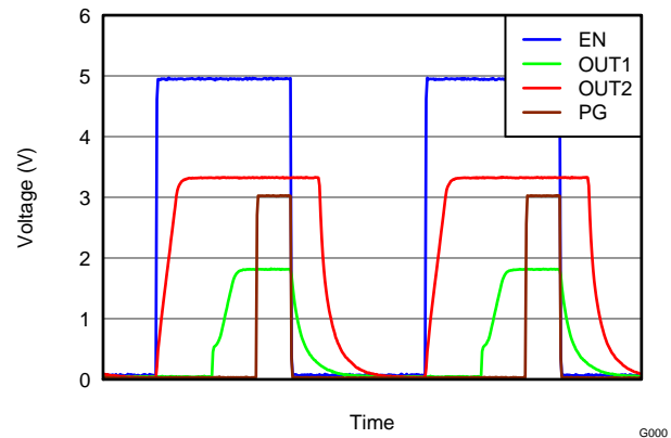
Figure 31. Power Sequence with SEQ = H
