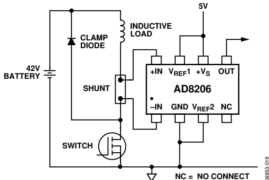
Figure 22. Low-Side Switch
