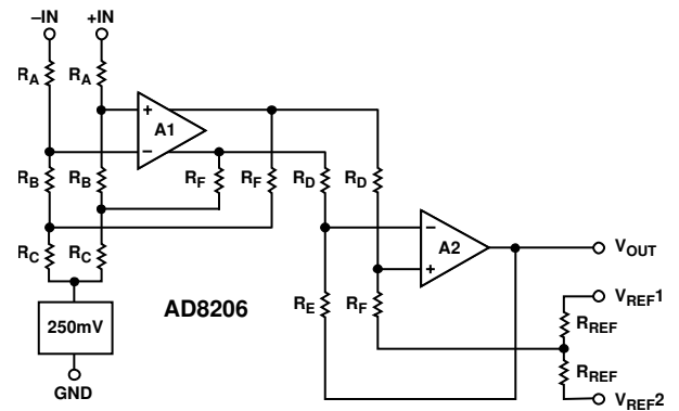
Figure 16. Simplified Schematic
