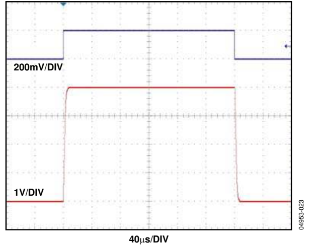
Figure 8. Rise/Fall Time
