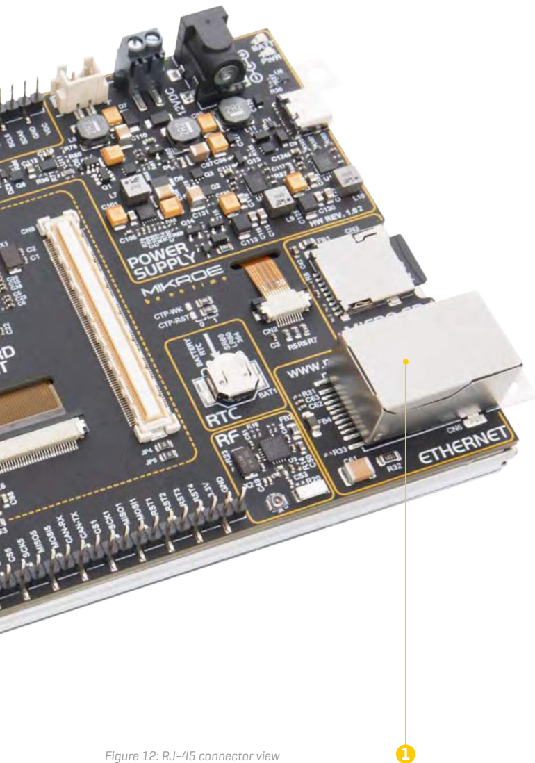
Figure 12: RJ-45 connector view
