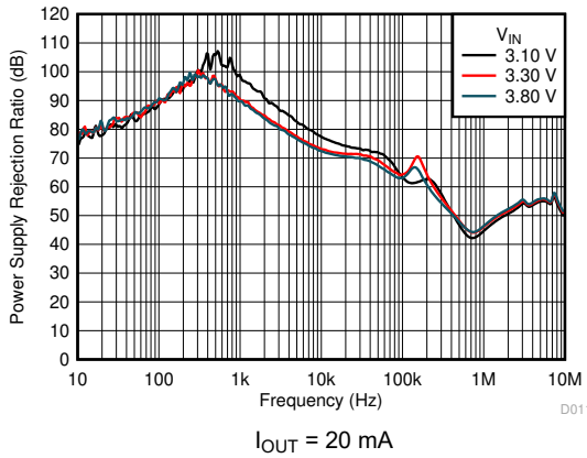
Figure 6-61. PSRR vs V_{IN} vs Frequency and V_{IN}
