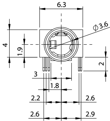
Unplugged Schematic
