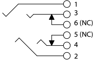
Unplugged Schematic
