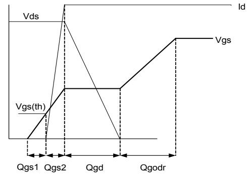
Fig 19. Gate Charge Waveform
