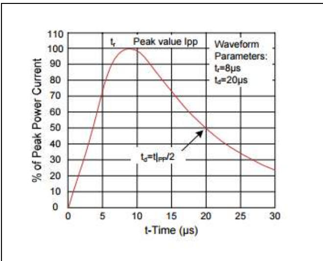
Figure 1. Pulse Waveform
