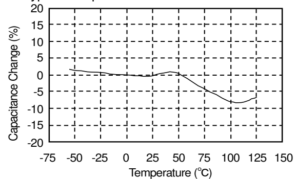
Typical temperature characteristics Char.R7 (X7R)
