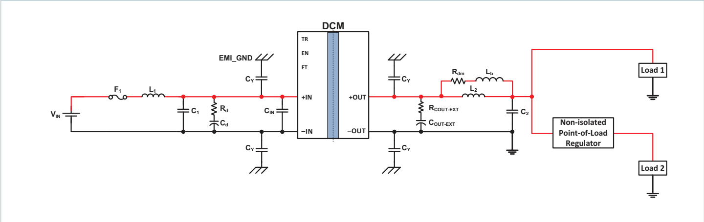
Typical Application 2: Single DCM4623xD2K31E0yzz, to a non-isolated regulator, and direct to load
