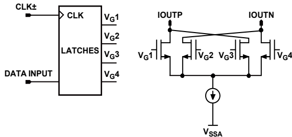
Figure 128. Quad-Switch Architecture
