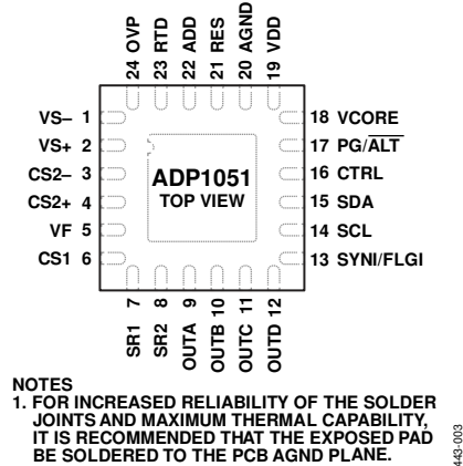
Figure 3. Pin Configuration
